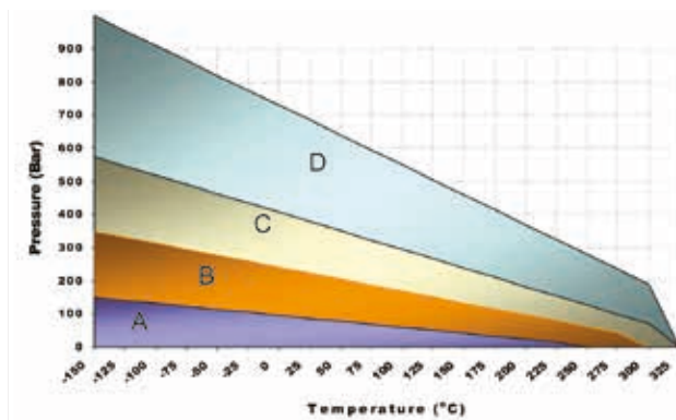
Figure 1, Temperature/Pressure Chart
